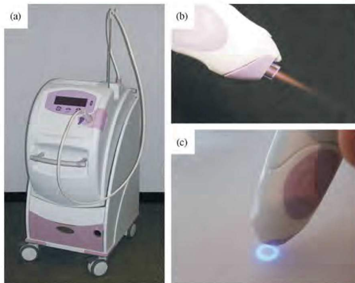
Figure 2 Plasma skin regeneration (PSR) using the Portrait® PSR. The plasma-generating device (a) and handpiece (b) with plasma energy emanating from tip are shown. Appearance of blue non-contact illuminated targeting ring used for gauging appropriate incident angle and distance from skin surface (c). (Modified and reproduced with permission from Rhytec, Inc.)
